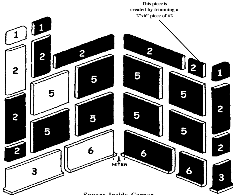
Square Inside Corner Installation with Round Outside Corners
